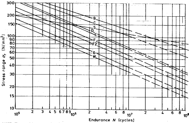
Fig. 15. Summary of mean-line \sigma_r - N curves
