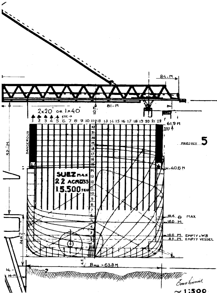
Fig. 1.6.1 Hatchless vessel, 22 across
