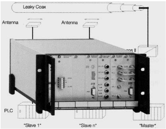
Fig. 9.6.2 Data transmission Powertrans® II
