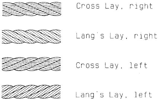
Fig. 2.4.1 Wire rope types
