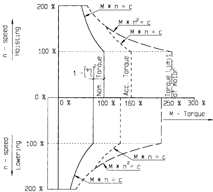
Fig. 3.1.6 AC frequency control: torque–speed diagram for hoisting/lowering
