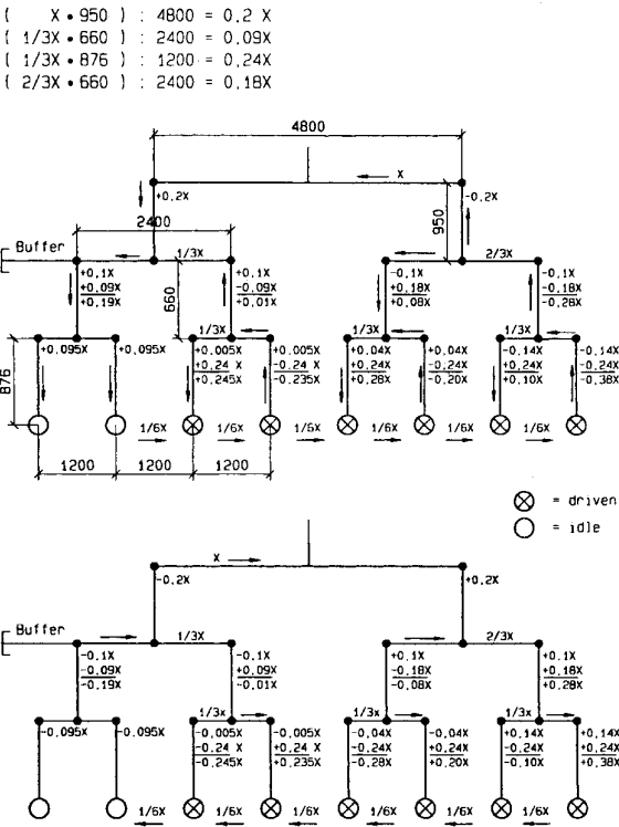
Fig. 8.3.2 Wheel load scheme through the horizontal force X
