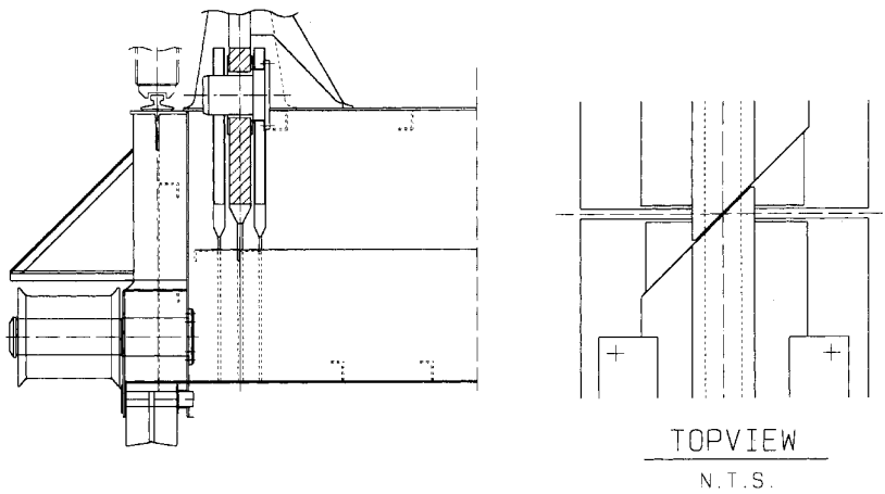
Fig. 8.5.4 Boom hinge point of a container crane
