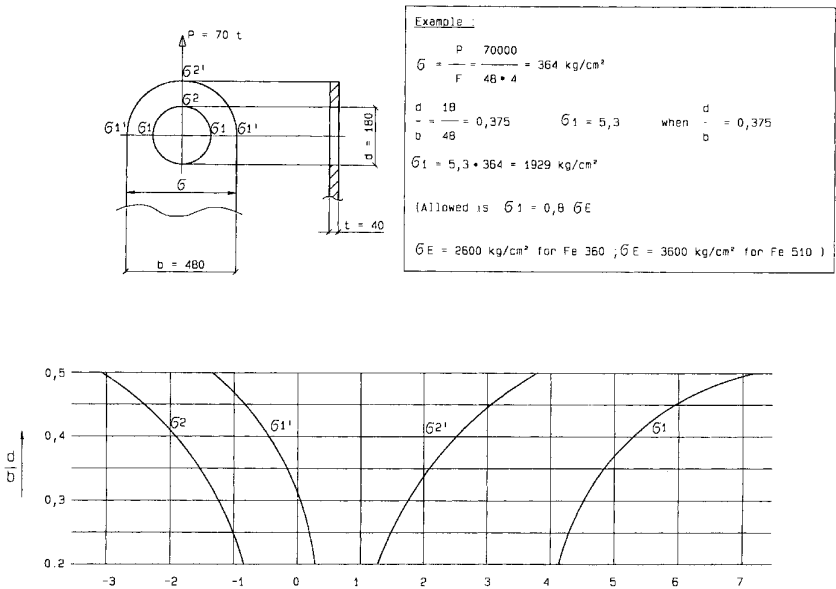
Fig. 7.5.1 The calculation of lugs according to Professor Bleich
