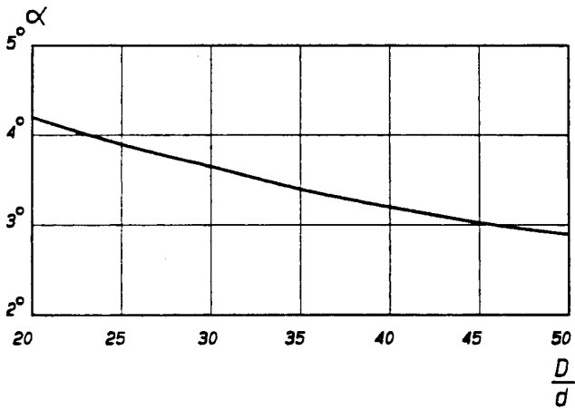
Fig. 2.5.2 Wire rope running off from the drum; maximum allowable deviation into the direction of the groove, measured from the tangent of the groove D =drum diameter, centre to centre of wire rope d =wire rope diameter
