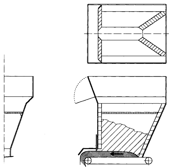
Fig. 9.7.1 Hopper with conveyor
