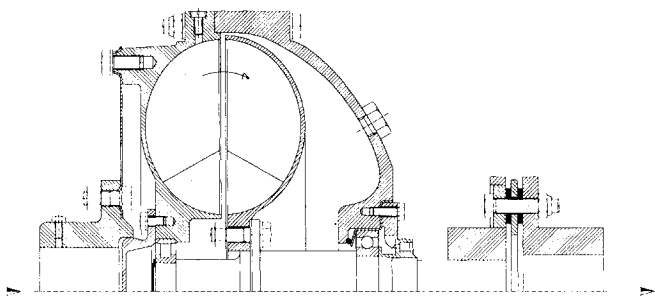
Fig. 3.1.2 Fluid coupling
