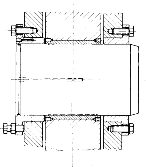
Fig. 8.5.6 Bronze bushed hinge point
