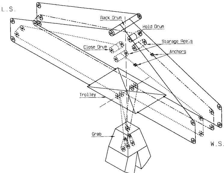
Fig. 6.1.5 ‘Fleet through’ reeving system
