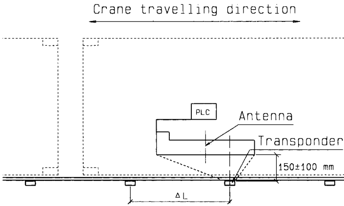
Fig. 6.7.6 Antenna-transponder system
