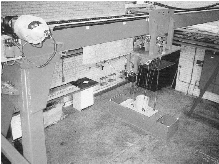
Fig. 6.11.2 The 1:15 scale working model
