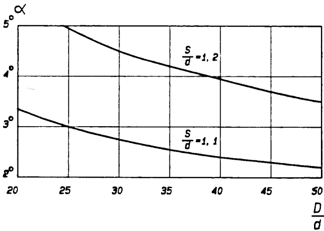
Fig. 2.5.3 Wire rope running off from the drum; maximum allowable deviation against the direction of the groove, measured from the tangent of the groove D =drum diameter, centre to centre of wire rope d =wire rope diameter S =pitch
