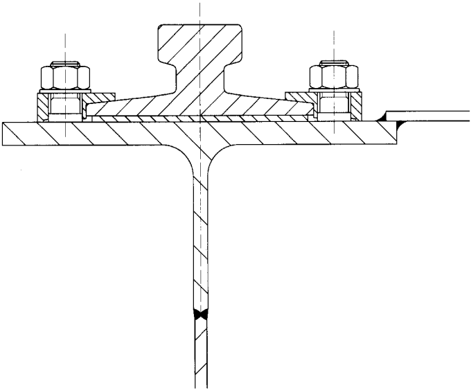
Fig. 8.5.1 Clipped trolley rail
